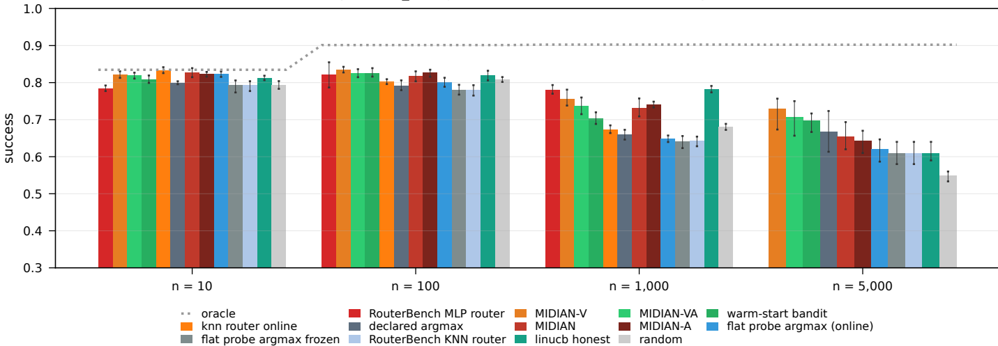
RouterEval real LLM pools, all_strong (10-1,000) + leaderboard (5,000), \beta = 0.25 , random liars
