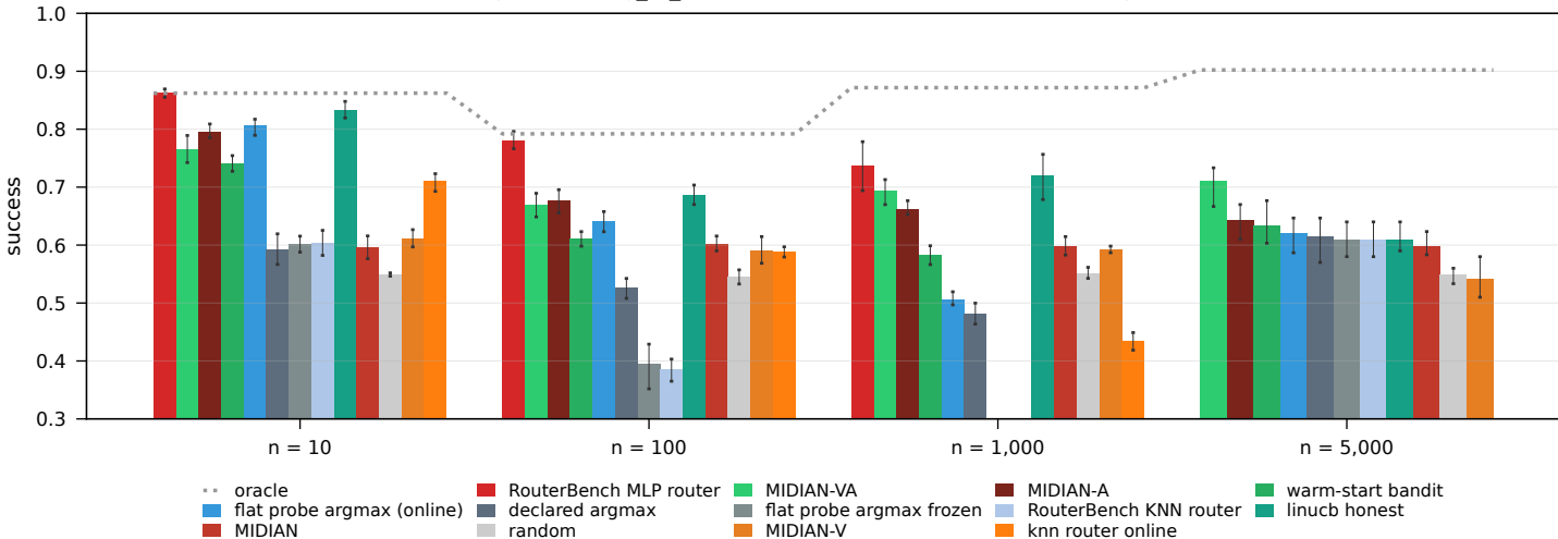
RouterEval real LLM pools, strong_to_weak (10-1,000) + leaderboard (5,000), \beta = 0.5 , low-skill cartel
