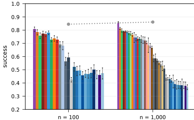
live RTE, specialist, \beta = 0.1 , random liars
