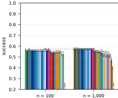
live RTE, bimodal, honest ( \beta = 0 )
