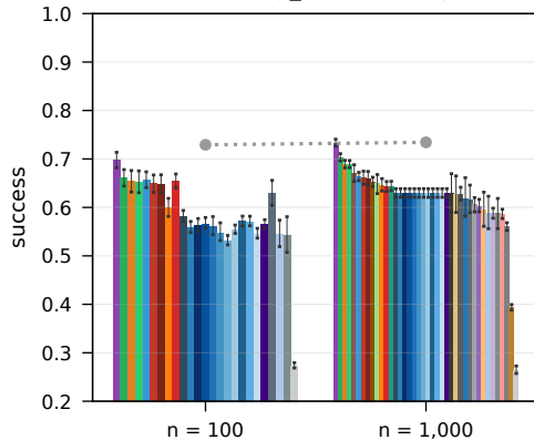
live RTE, heavy_tail, honest ( \beta = 0 )
