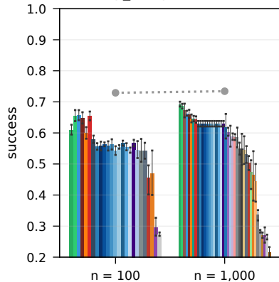
live RTE, heavy_tail, \beta = 0.5 , low-skill cartel
