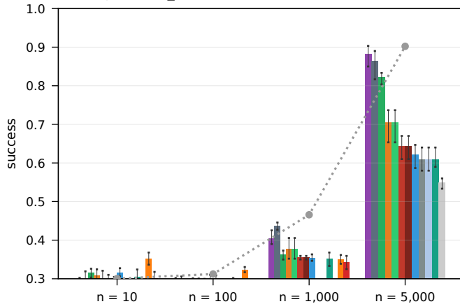
RouterEval real LLM pools, all_weak (10-1,000) + leaderboard (5,000), honest ( \beta = 0 )
