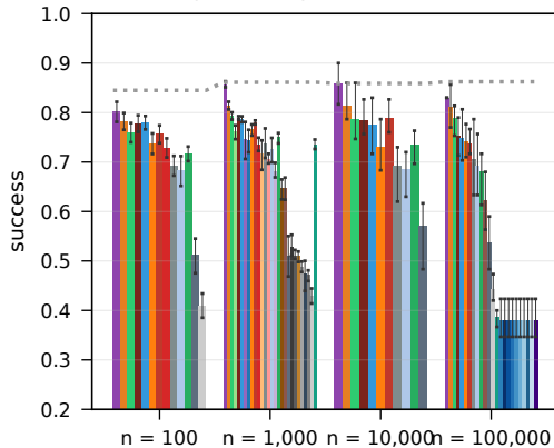
live RTE, specialist, \beta = 0.25 , low-skill cartel
