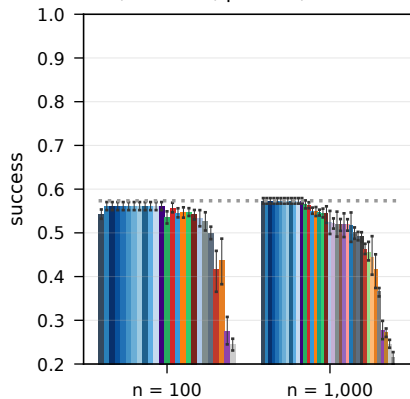
live RTE, bimodal, \beta = 0.5 , low-skill cartel
