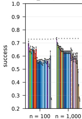
live RTE, heavy_tail, \beta = 0.1 , random liars
