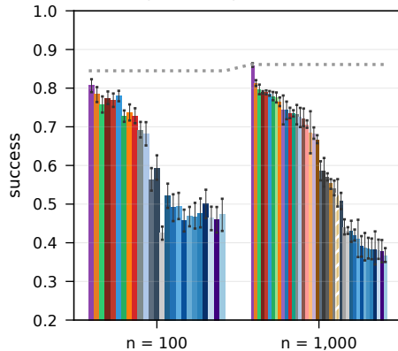
live RTE, specialist, \beta = 0.1 , random liars
