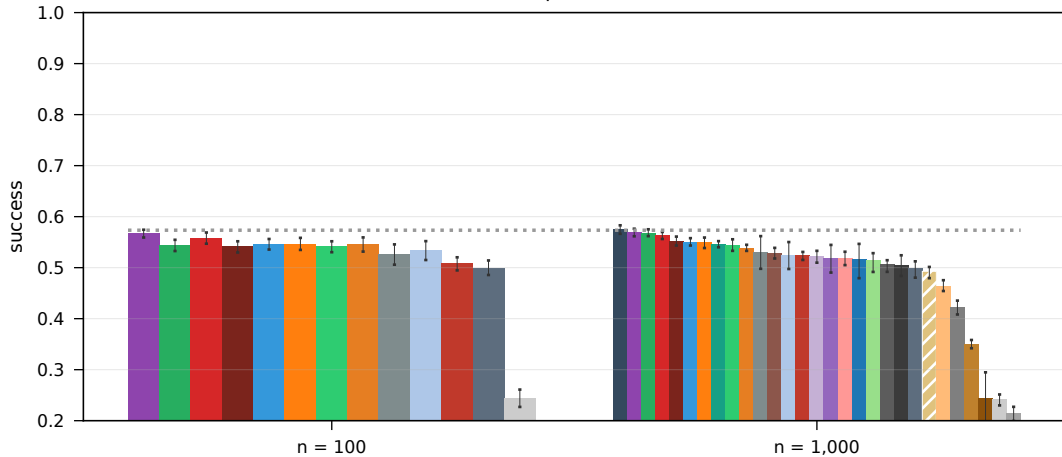
live RTE, bimodal, \beta = 0.25 , low-skill cartel
