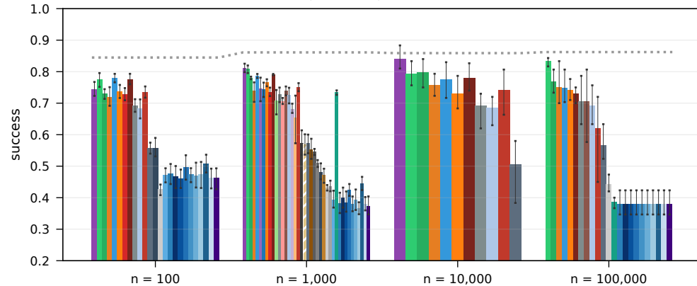
live RTE, specialist, \beta = 0.5 , random liars
