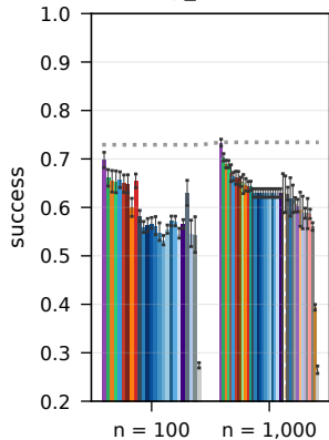
live RTE, heavy_tail, honest ( \beta = 0 )
