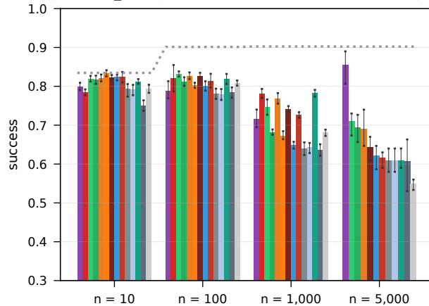
RouterEval real LLM pools, all_strong (10-1,000) + leaderboard (5,000), \beta = 0.25 , low-skill cartel
