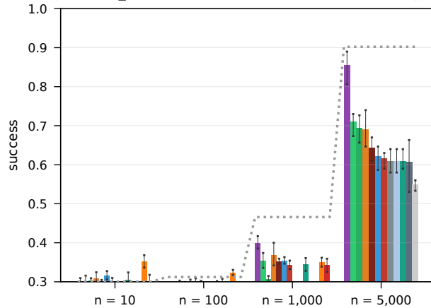
RouterEval real LLM pools, all_weak (10-1,000) + leaderboard (5,000), \beta = 0.25 , low-skill cartel
