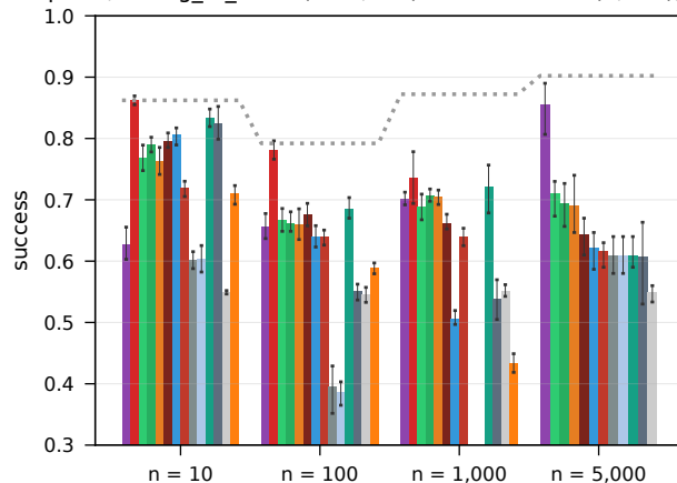
RouterEval real LLM pools, strong_to_weak (10-1,000) + leaderboard (5,000), \beta = 0.25 , low-skill cartel
