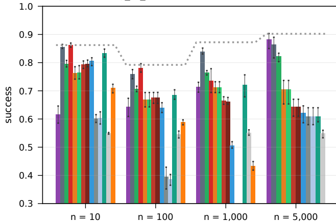
RouterEval real LLM pools, strong_to_weak (10-1,000) + leaderboard (5,000), honest ( \beta = 0 )
