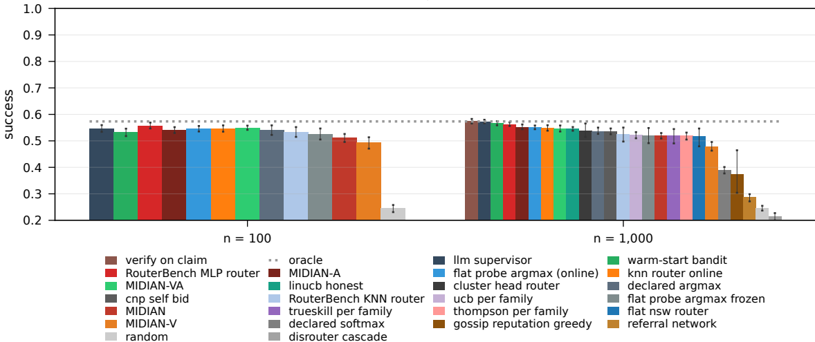
live RTE, bimodal, \beta = 0.5 , random liars
