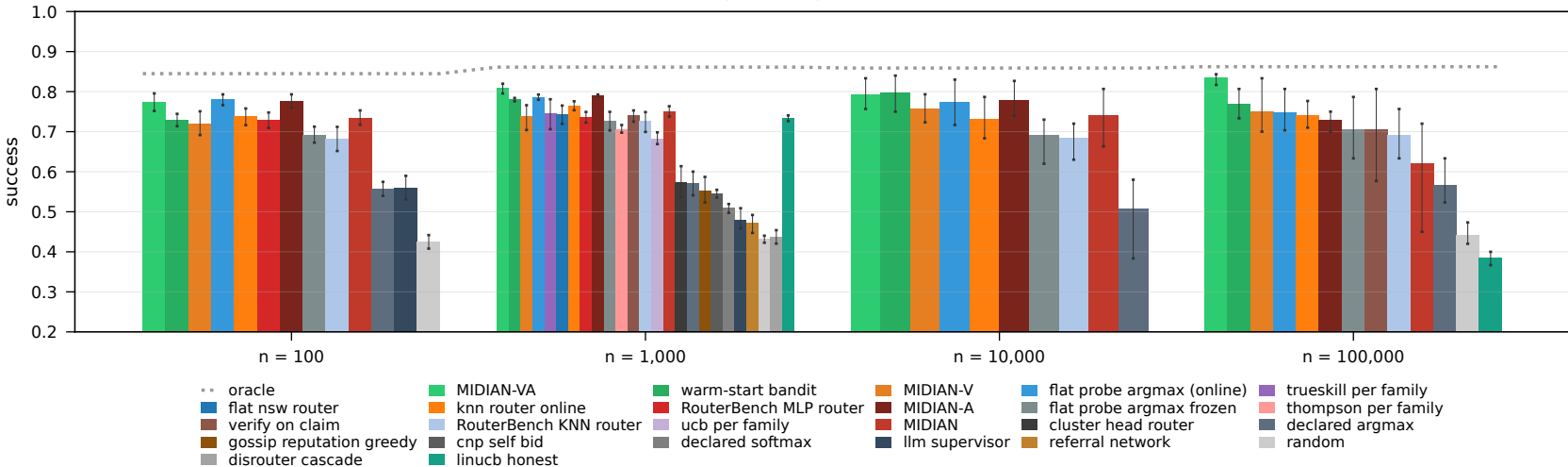
live RTE, specialist, \beta = 0.5 , random liars
