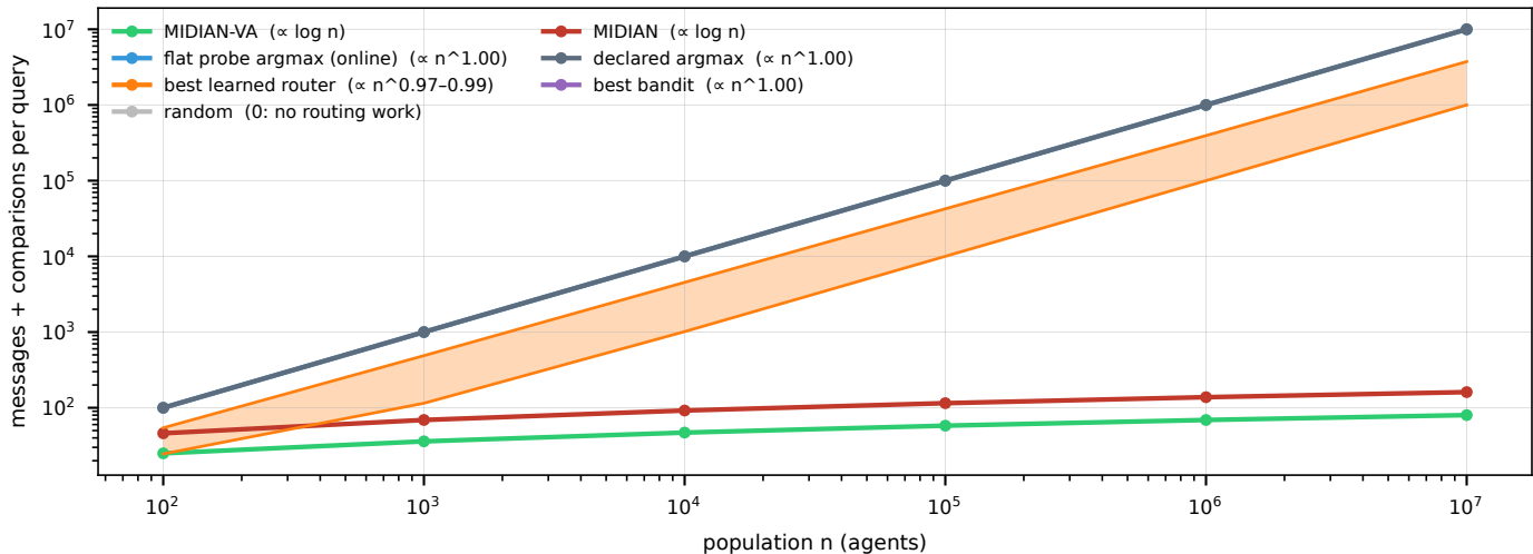
C routing work per query, the arms of A / B: MIDIAN grows like \log n (calibrated bernoulli, b = 3 , exact ledger)
