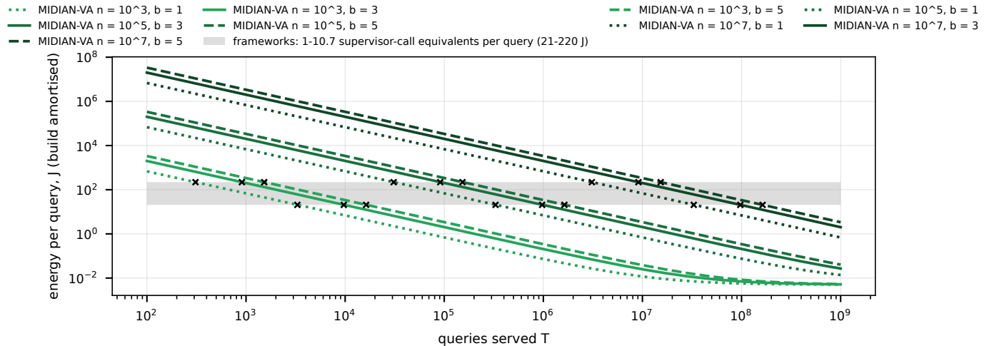
D energy per query (*): MIDIAN-VA pays one probing build, then \sim 0.01 J / query; frameworks pay supervisor LLM calls every query
