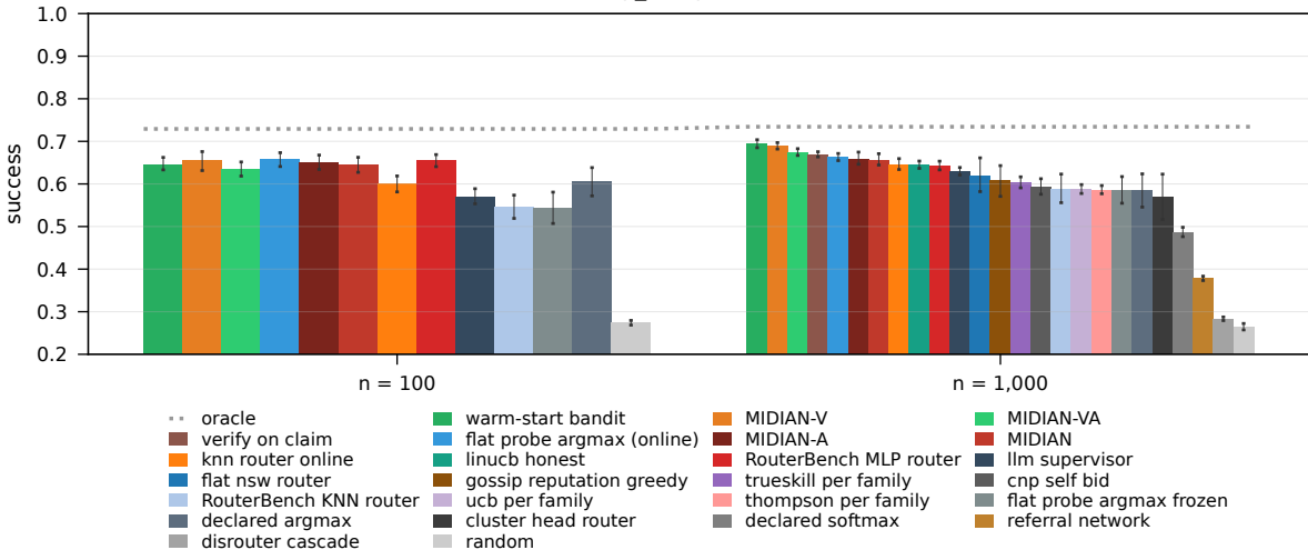
live RTE, heavy_tail, \beta = 0.1 , random liars
