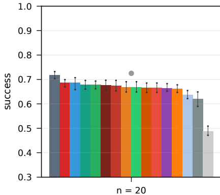
LLMRouterBench 20-model pool, honest ( \beta = 0 )
