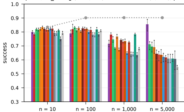
RouterEval real LLM pools, all_strong (10-1,000) + leaderboard (5,000), \beta = 0.25 , low-skill cartel
