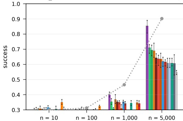
RouterEval real LLM pools, all_weak (10-1,000) + leaderboard (5,000), \beta = 0.25 , low-skill cartel
