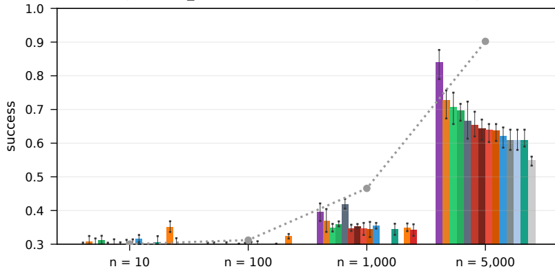
RouterEval real LLM pools, all_weak (10-1,000) + leaderboard (5,000), \beta = 0.25 , random liars
