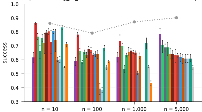
RouterEval real LLM pools, strong_to_weak (10-1,000) + leaderboard (5,000), \beta = 0.5 , random liars
