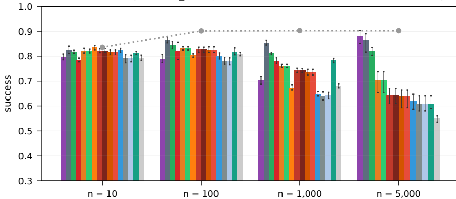
RouterEval real LLM pools, all_strong (10-1,000) + leaderboard (5,000), honest ( \beta = 0 )
