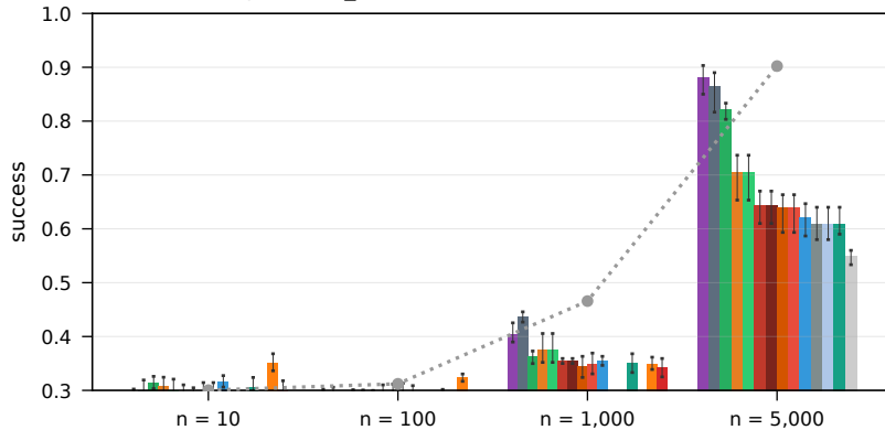
RouterEval real LLM pools, all_weak (10-1,000) + leaderboard (5,000), honest ( \beta = 0 )
