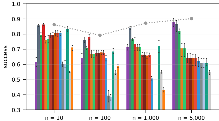
RouterEval real LLM pools, strong_to_weak (10-1,000) + leaderboard (5,000), honest ( \beta = 0 )
