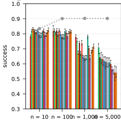
RouterEval real LLM pools, all_strong (10-1,000) + leaderboard (5,000), \beta = 0.5 , low-skill cartel
