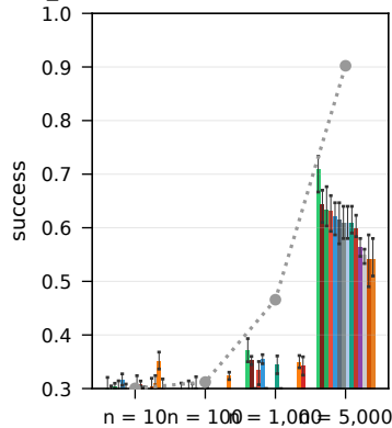
RouterEval real LLM pools, all_weak (10-1,000) + leaderboard (5,000), \beta = 0.5 , low-skill cartel
