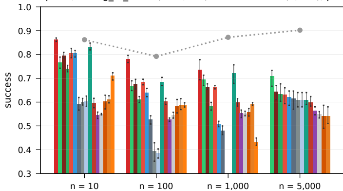
RouterEval real LLM pools, strong_to_weak (10-1,000) + leaderboard (5,000), \beta = 0.5 , low-skill cartel
