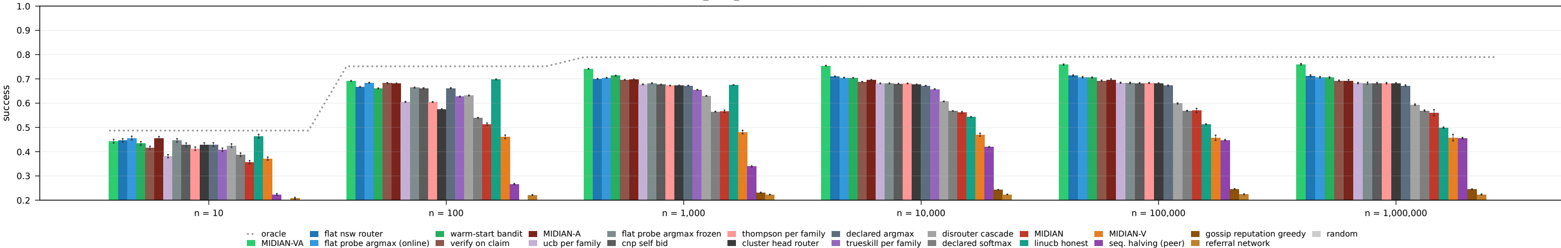
replay (replay_scale_v5), all shapes pooled, \beta = 0.5 , low-skill cartel
