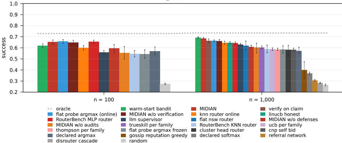
live RTE, heavy_tail, \beta = 0.5 , random liars
