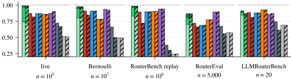
success relative to oracle
