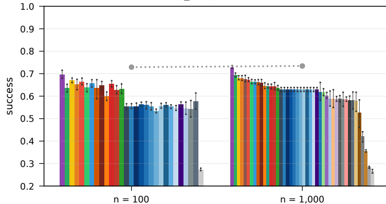
live RTE, heavy_tail, \beta = 0.25 , random liars
