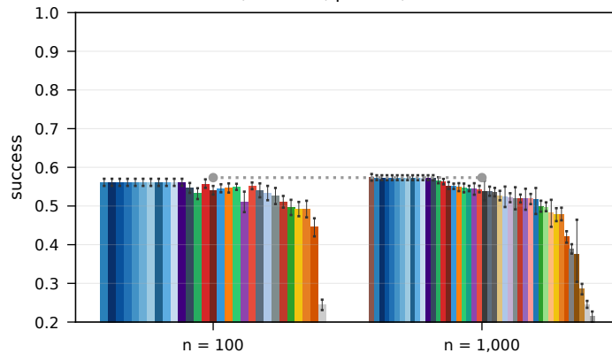
live RTE, bimodal, \beta = 0.5 , random liars
