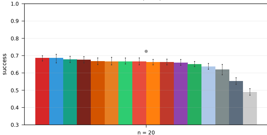
LLMRouterBench 20-model pool, \beta = 0.25 , low-skill cartel
