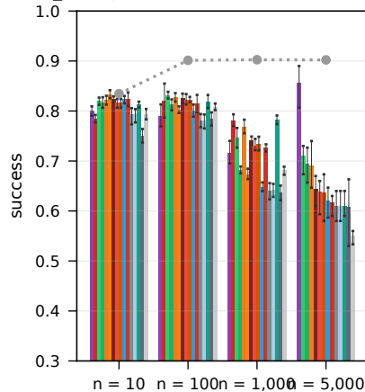
RouterEval real LLM pools, all_strong (10-1,000) + leaderboard (5,000), \beta = 0.25 , low-skill cartel
