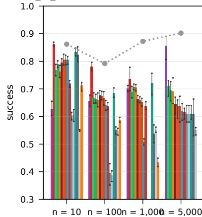
RouterEval real LLM pools, strong_to_weak (10-1,000) + leaderboard (5,000), \beta = 0.25 , low-skill cartel
