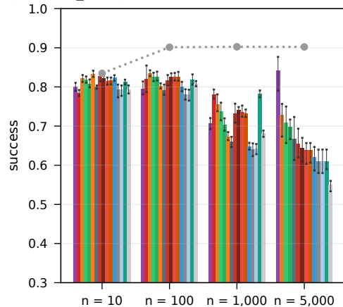
RouterEval real LLM pools, all_strong (10-1,000) + leaderboard (5,000), \beta = 0.25 , random liars
