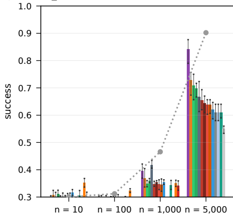
RouterEval real LLM pools, all_weak (10-1,000) + leaderboard (5,000), \beta = 0.25 , random liars
