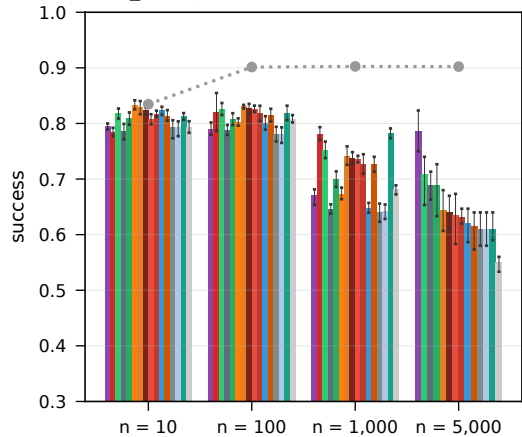
RouterEval real LLM pools, all_strong (10-1,000) + leaderboard (5,000), \beta = 0.5 , random liars
