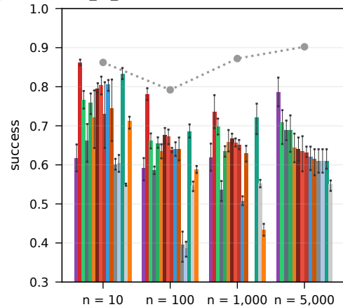
RouterEval real LLM pools, strong_to_weak (10-1,000) + leaderboard (5,000), \beta = 0.5 , random liars
