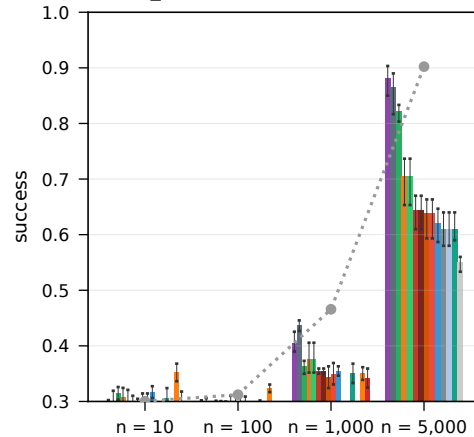
RouterEval real LLM pools, all_weak (10-1,000) + leaderboard (5,000), honest ( \beta = 0 )
