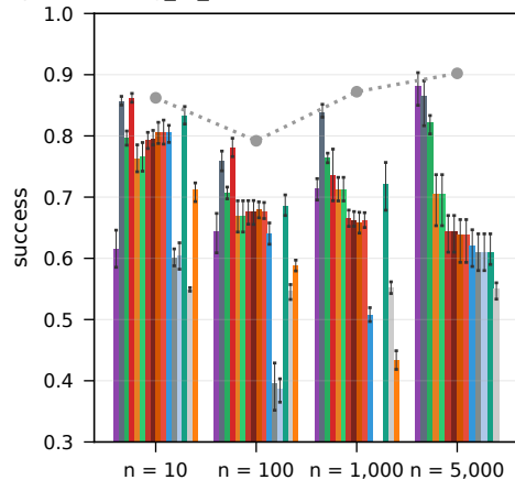
RouterEval real LLM pools, strong_to_weak (10-1,000) + leaderboard (5,000), honest ( \beta = 0 )
