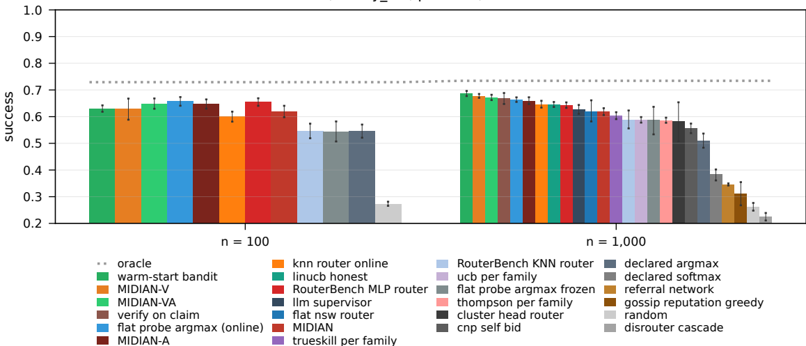
live RTE, heavy_tail, \beta = 0.25 , low-skill cartel
