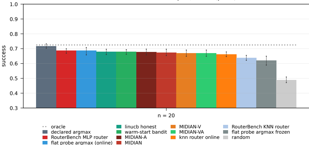
LLMRouterBench 20-model pool, honest ( \beta = 0 )
